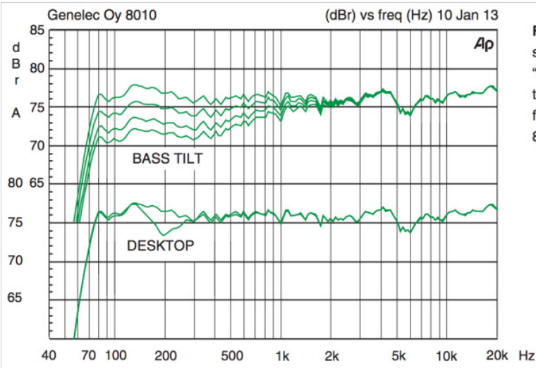
Figure 4. The curves show the effect of the “Bass Tilt” and “Desktop” controls on the free field response of the 8010A
